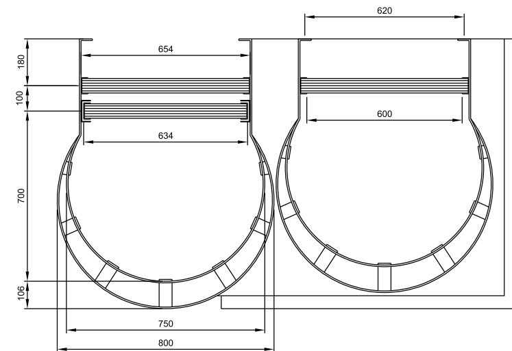
CAT LADDER PLAN WITH INTERMEDIATE LANDING (PARAPET PLATFORM & RETURN LADDER ARE OMITTED FOR CLARITY)
