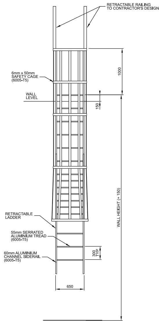
FIRE ESCAPE CAT LADDER 1:25
