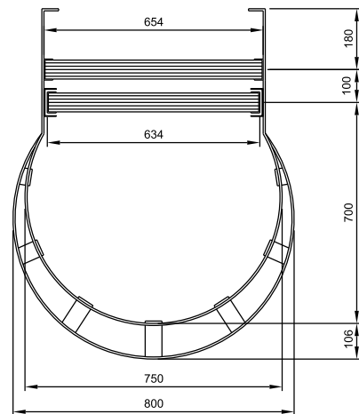
CAT LADDER PLAN (PARAPET PLATFORM & RETURN LADDER ARE OMITTED FOR CLARITY)
